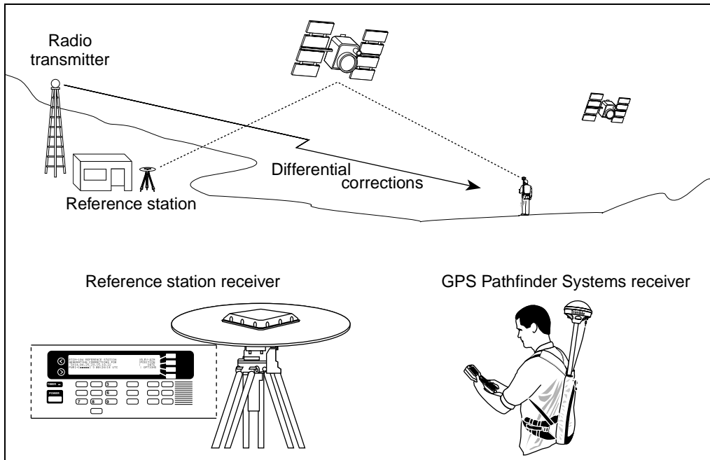
Figure 3.1 Components of a DGPS system
